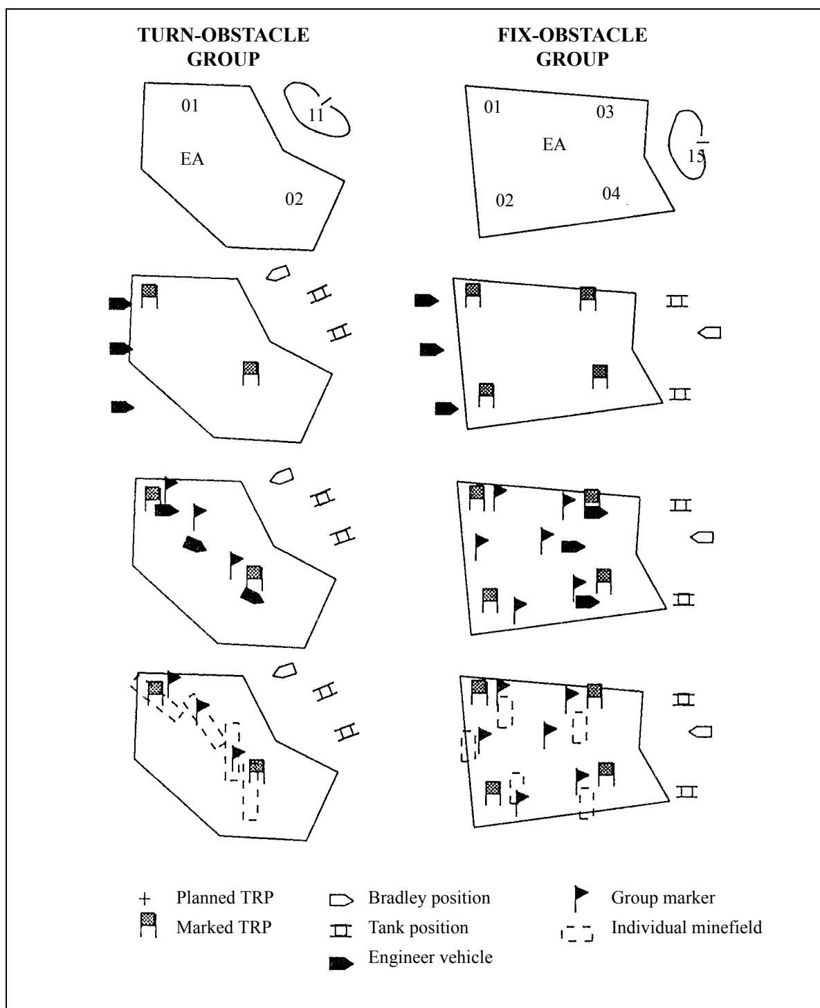
Figure 2-18. Minefield siting
