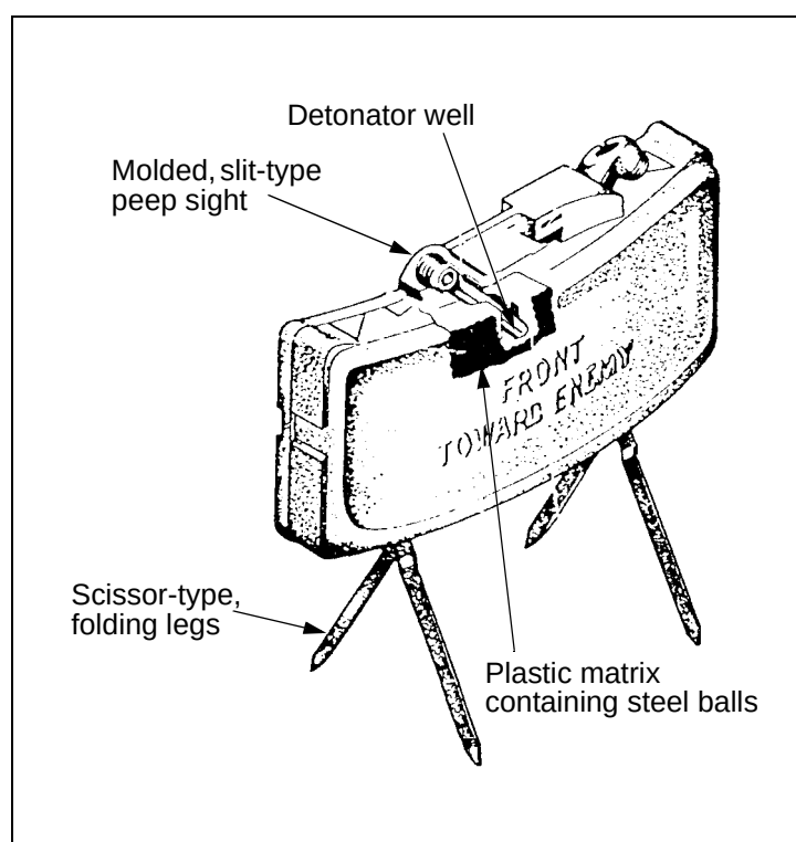
Figure 4-2. M18A1 claymore
