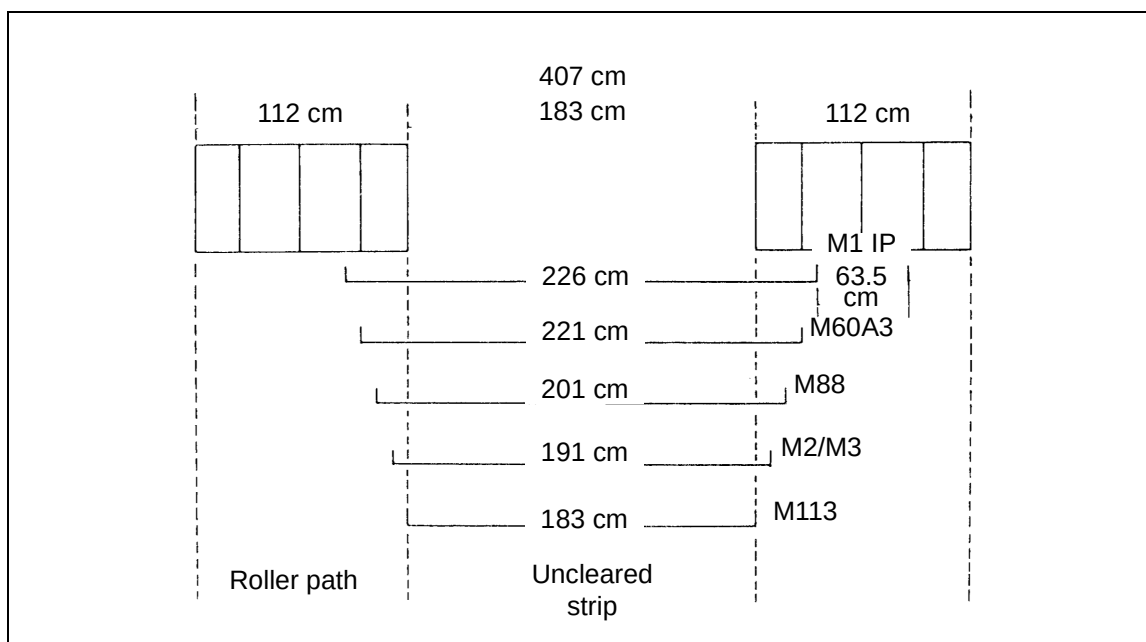
Figure 10-15. Mine-roller width compared to track-vehicle widths
