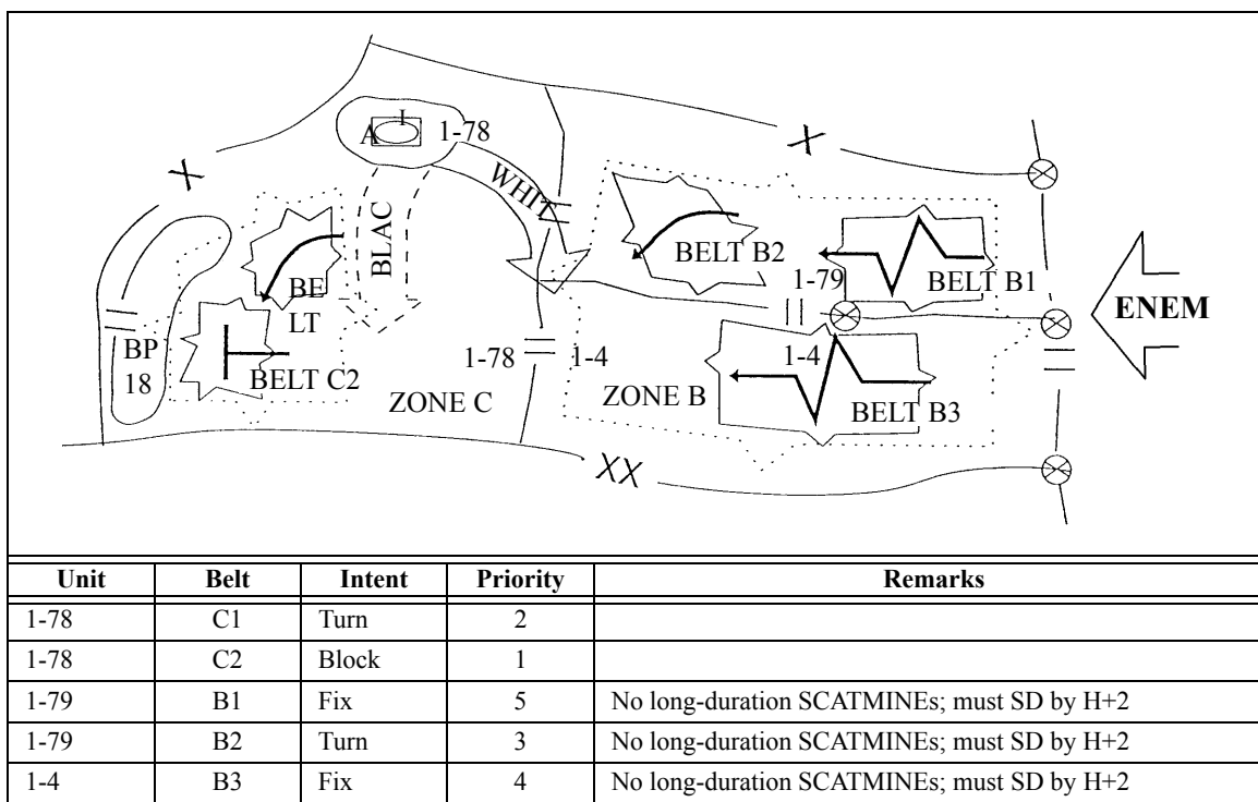
Figure 2-10. Obstacle belts
