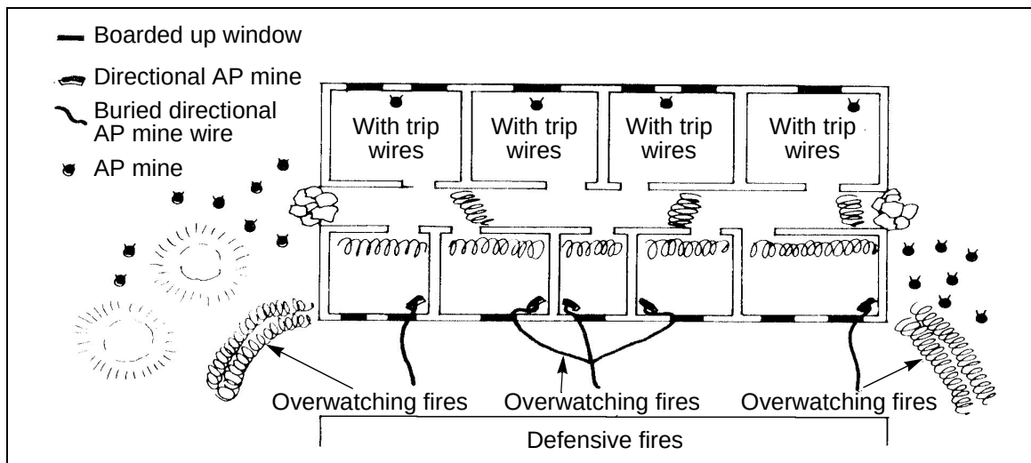
Figure 12-8. Building obstacles
